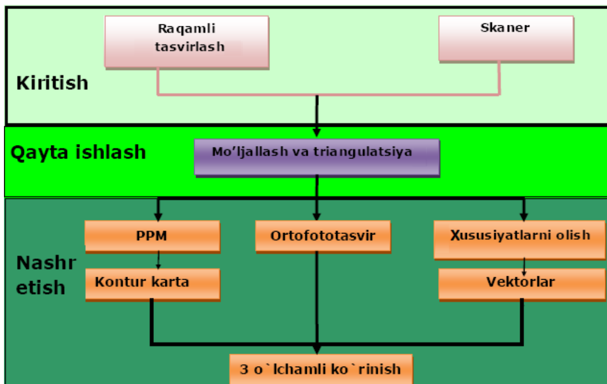
4.2-rasm. Anʼanaviy fotogrammetrik jarayon (Manba: Internet)
