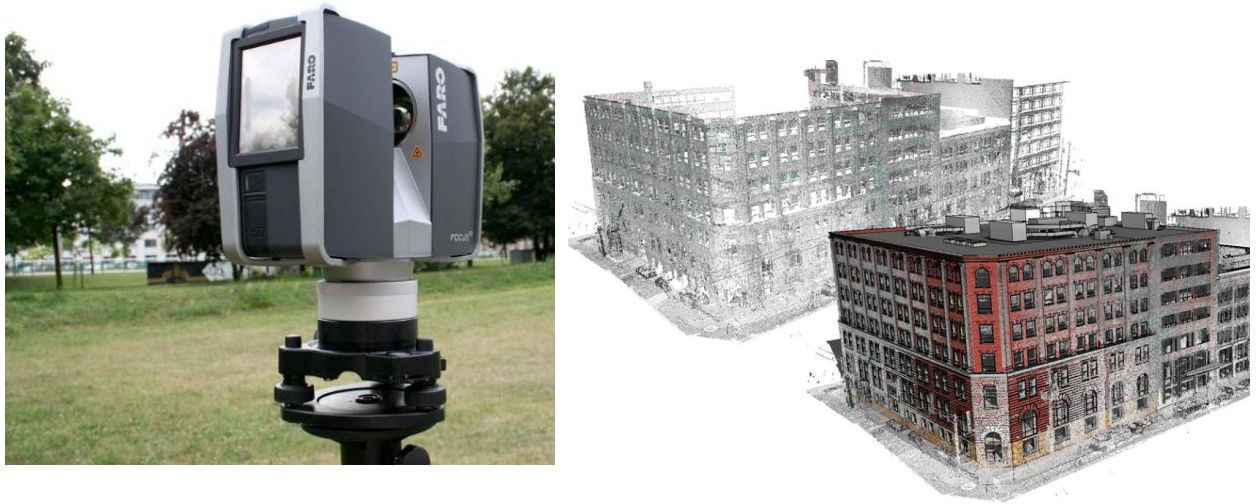
1.4-rasm. Uch o'lchamli lazer skaner (TX5 Trimble) va uning yordamida olingan tasvir (Manba: Internet)
