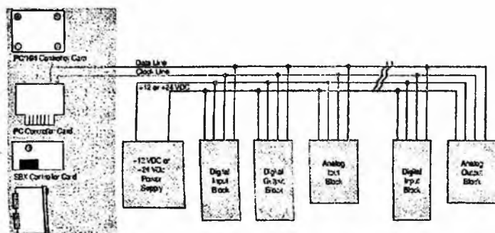
16.7-rasm. Seriplex tizimiga misol.
