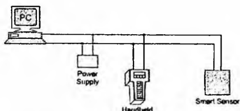
15.2-rasm. HART protokolidan nuqtadan nuqtagacha aloqa.
