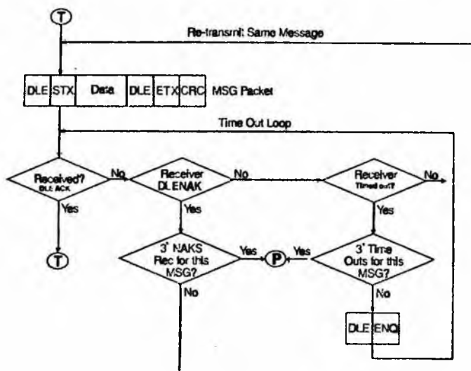
14.4-rasm. Protokolning tuzilishi.
