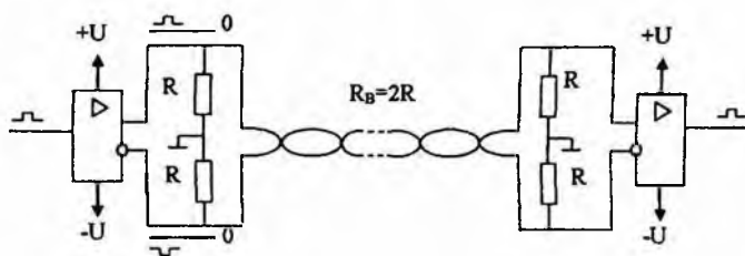
6.7-rasm. O'ralgan juftlikdan signalni differensial uzatish.
