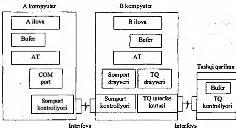
9.8-rasm. Tarmoqda masofadagi printerdan foydalanish.
