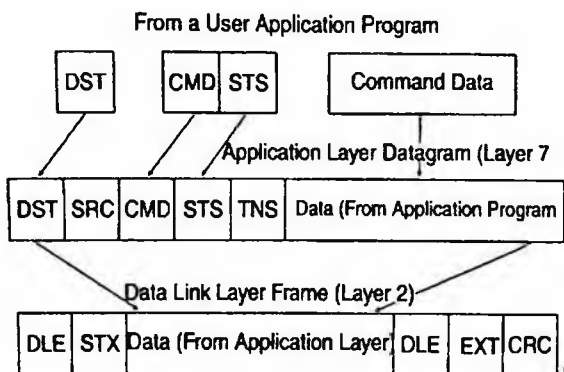
14.4-rasm. Protokolning tuzilishi.
