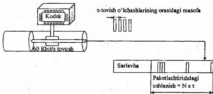
10.9-rasm. Paketlashtirishdagi ushlanish.
