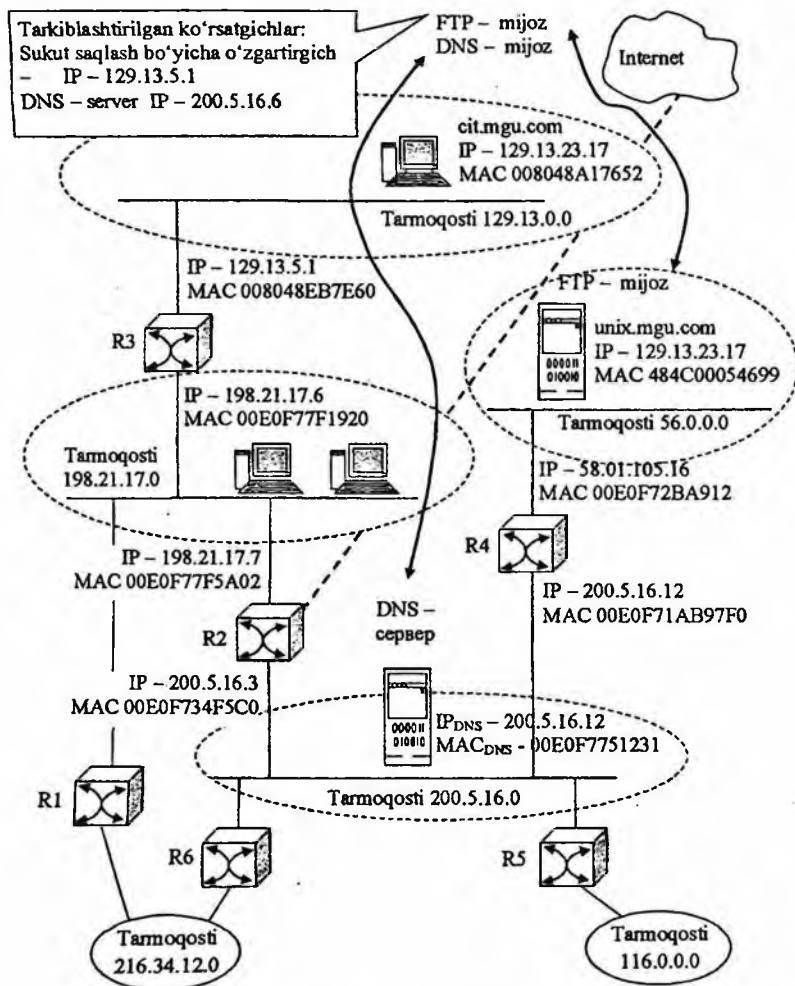
8.10-rasm. IP-yo'naltirishga misol.
