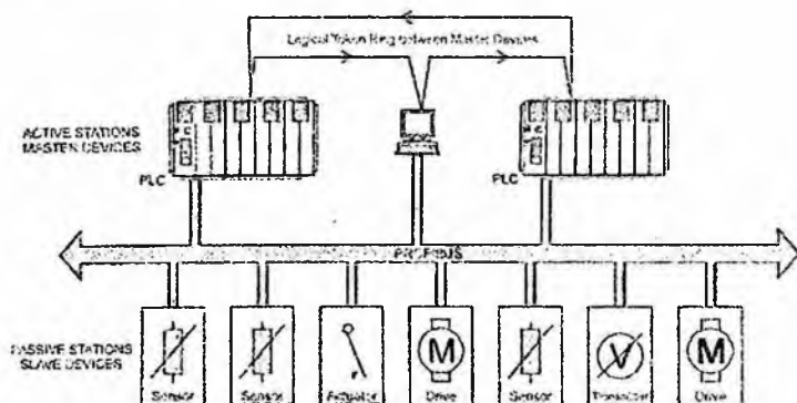
16.12-rasm. Profiliniyanning sodda tuzulishi.
